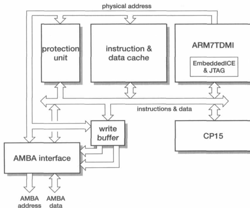
Figure 12.4 ARM740T organization.
