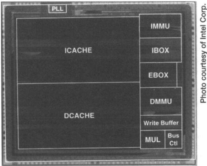
Figure 12.10 StrongARM die photograph.
