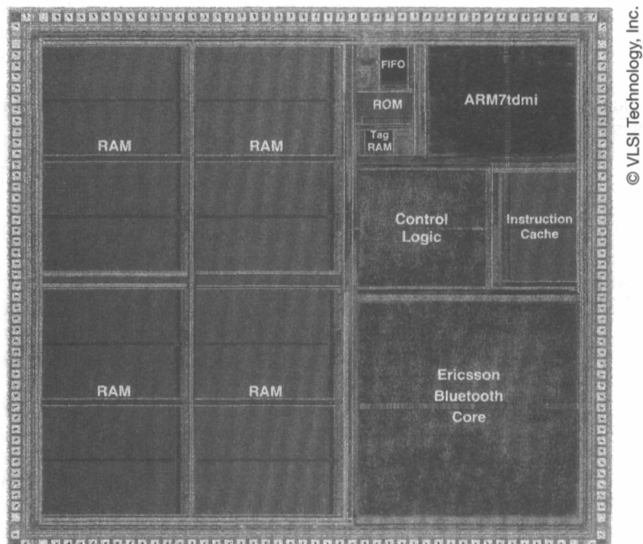
Figure 13.9 Bluetooth Baseband Controller die photograph.
