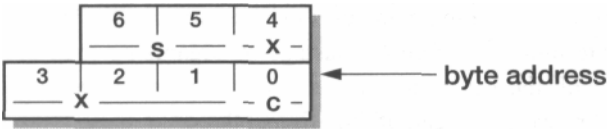
Figure 6.17 An example of packed struct memory allocation.
