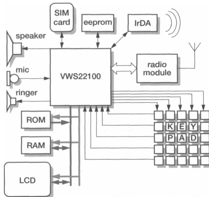
Figure 13.6 Typical GSM handset architecture.
