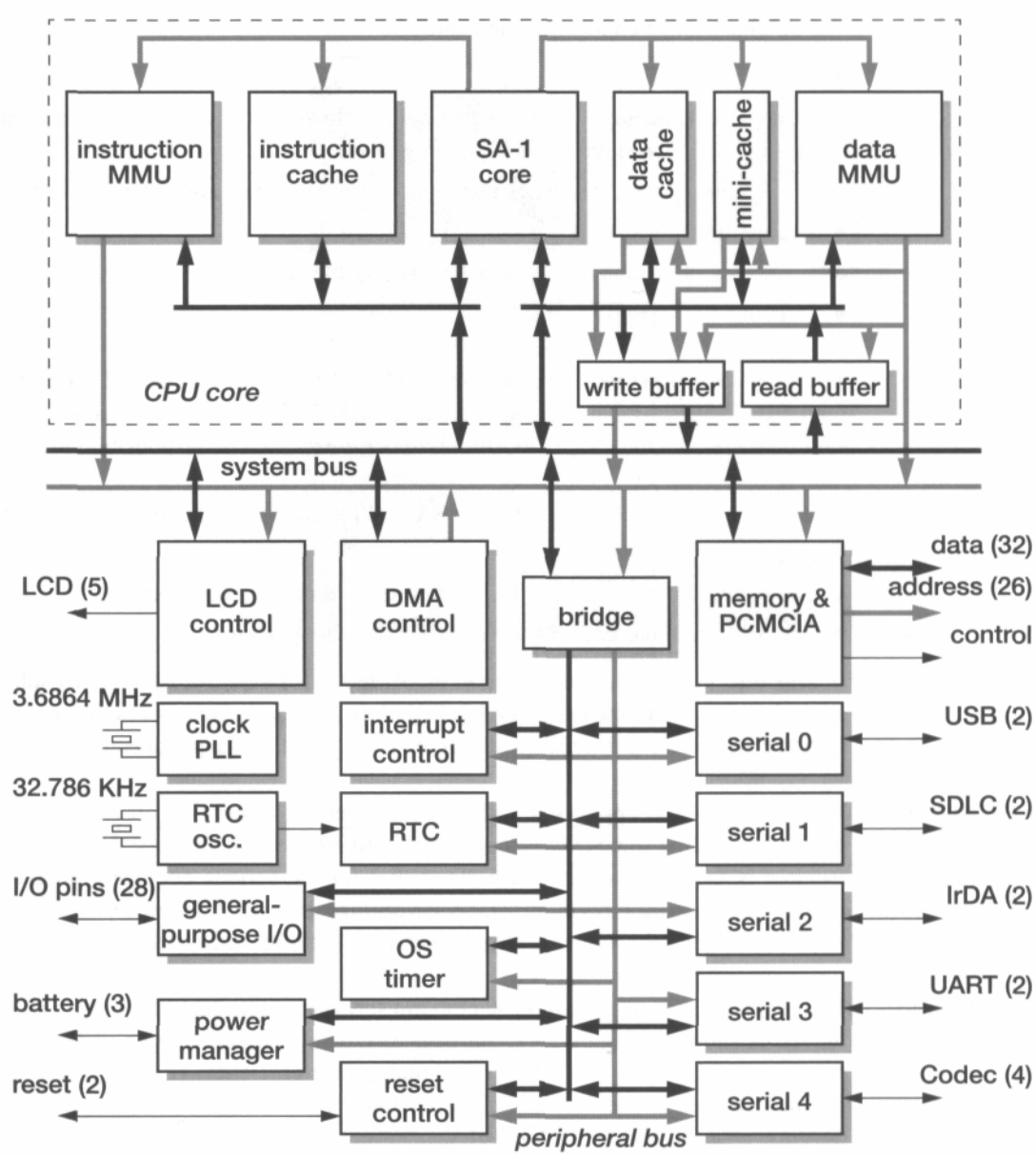
Figure 13.16 SA-1100 organization.
