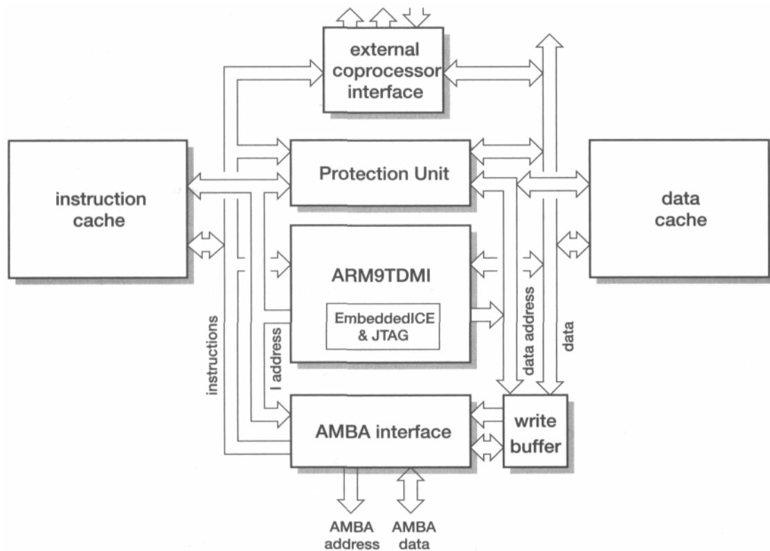
Figure 12.12 ARM940T organization.
