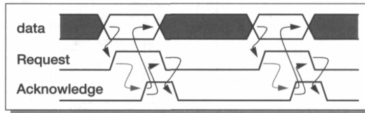
Figure 14.2 Level-signalling communication protocol.
