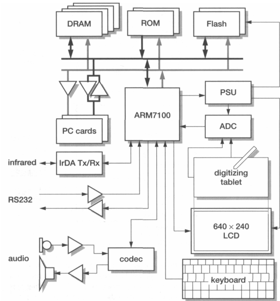
Figure 13.14 The Psion Series 5 hardware organization.
