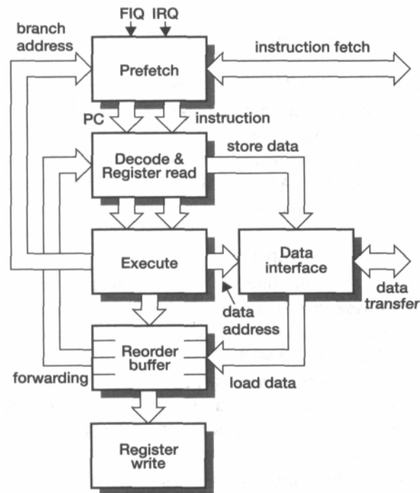
Figure 14.10 AMULETS core organization.
