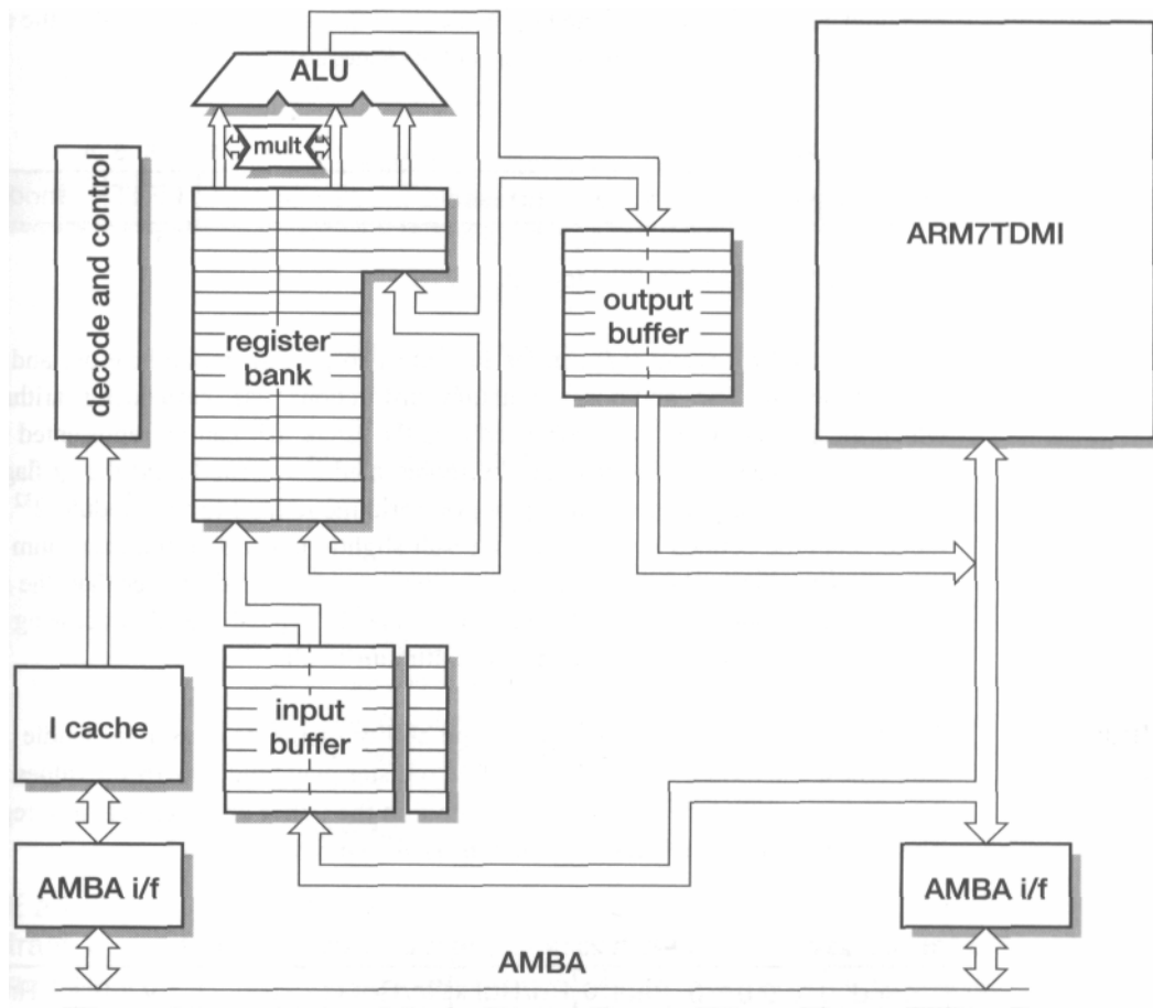
Figure 8.20 Piccolo organization.
