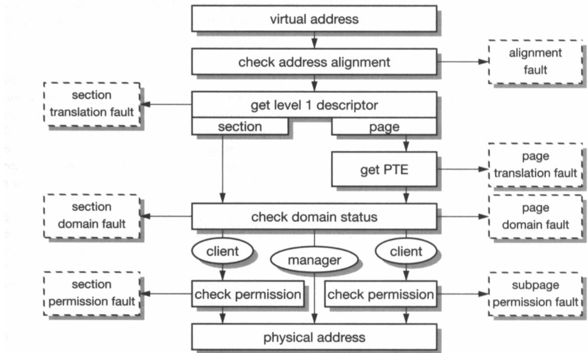
Figure 11.6 Access permission checking scheme.
