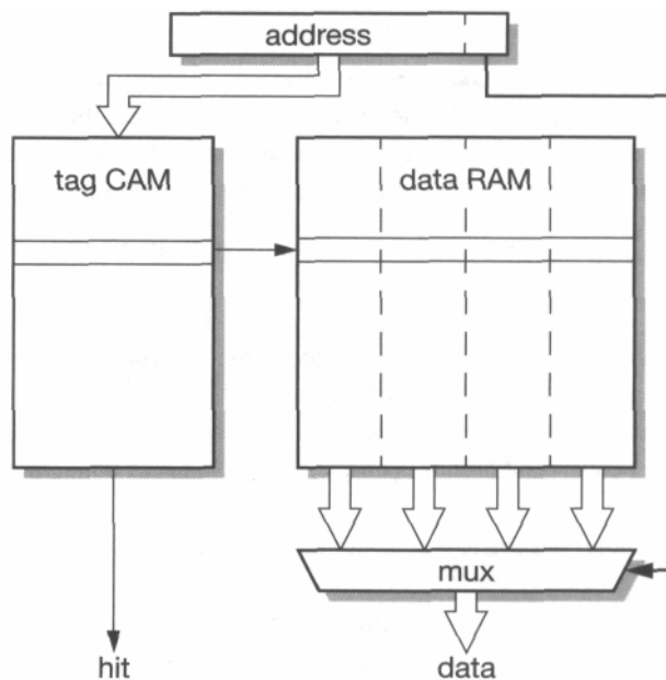
Figure 10.5 Fully associative cache organization.
