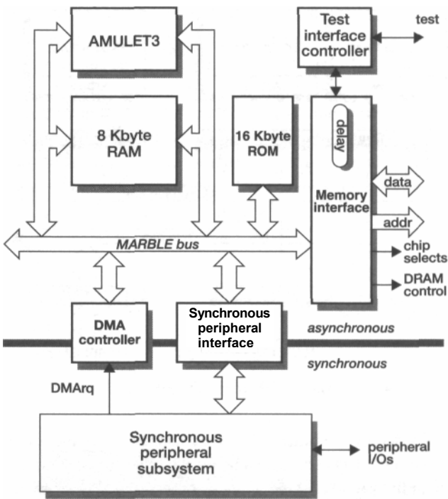
Figure 14.12 The AMULET3H asynchronous subsystem.
