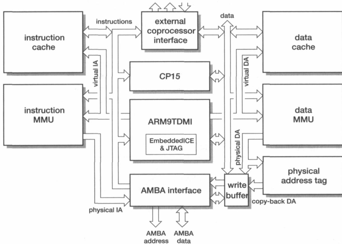
Figure 12.11 ARM920T organization.
