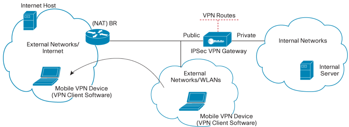
Figure 2. VPN Architecture
